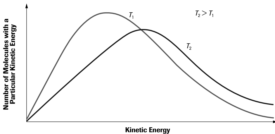
Kinetic Energy Distribution at Two Temperatures
