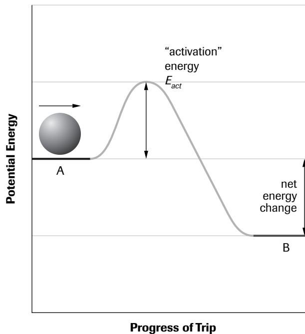
An Analogy for Activation Energy
