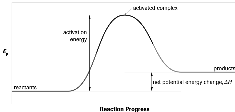
Potential Energy Changes During an Endothermic Reaction
