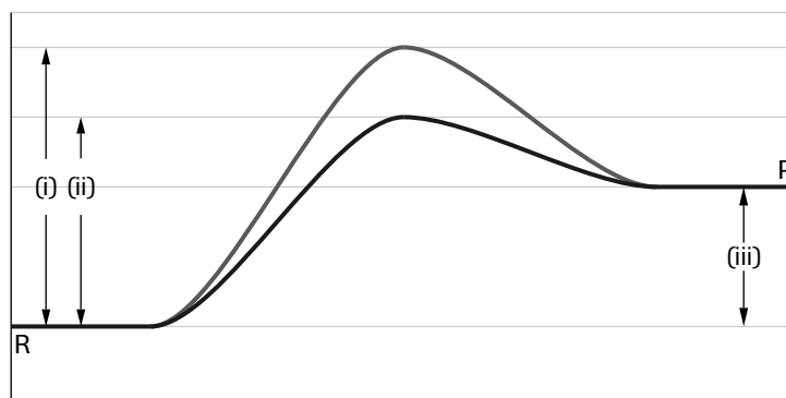
Potential Energy Diagram for System R→P
