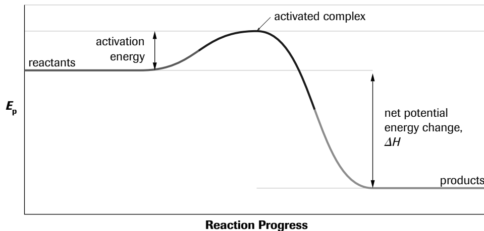
Potential Energy Changes During an Exothermic Reaction
